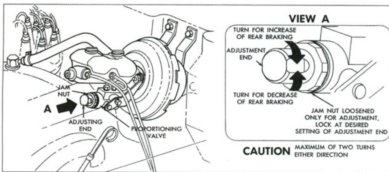
Fig. 3—1966 Corvette Heavy Duty Brakes (RPO J56)
