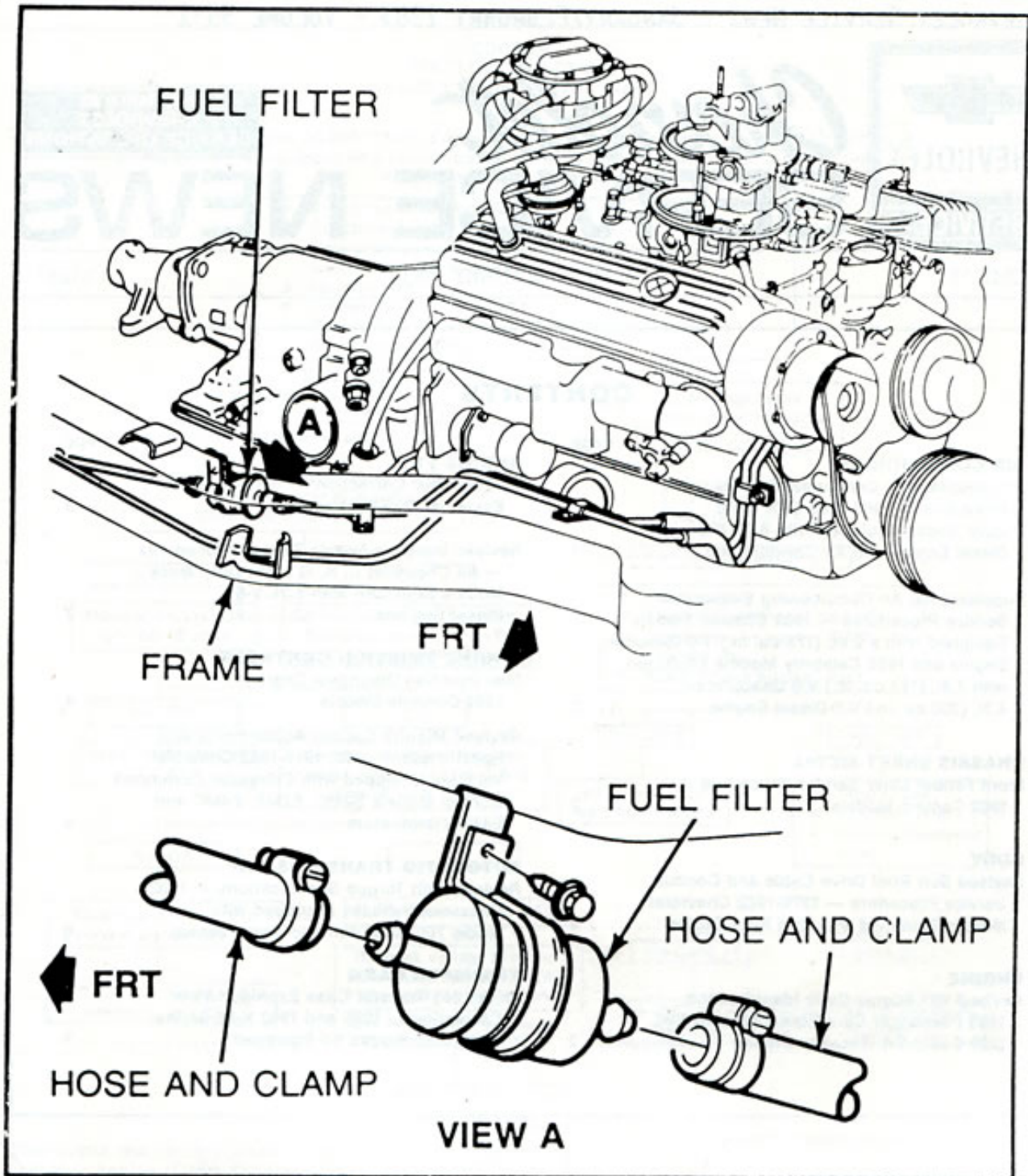
Fig. 1 — Fuel Filter
