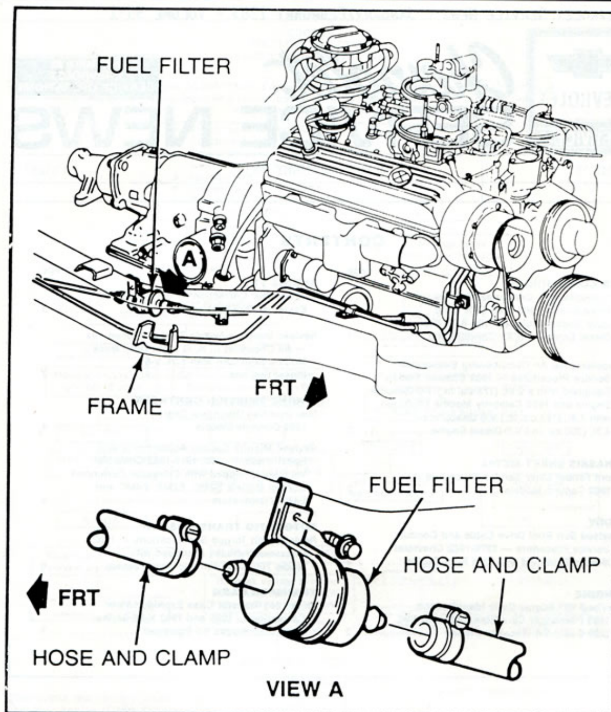
Fig. 1 — Fuel Filter
