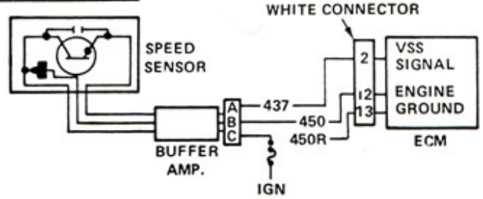
Fig. 2 — TC 24-Vehicle Speed Sensor
