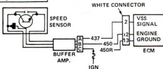
Fig. 2 — TC 24-Vehicle Speed Sensor
