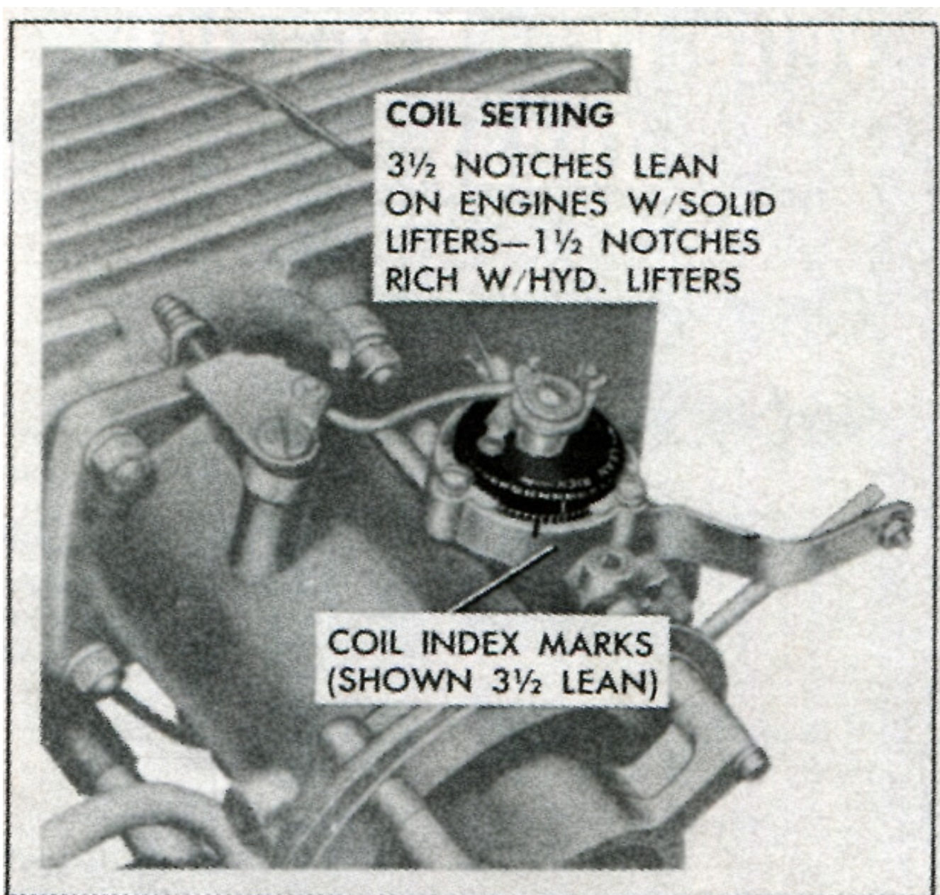
Fig. 2—Fuel Injection Cold Enrichment
