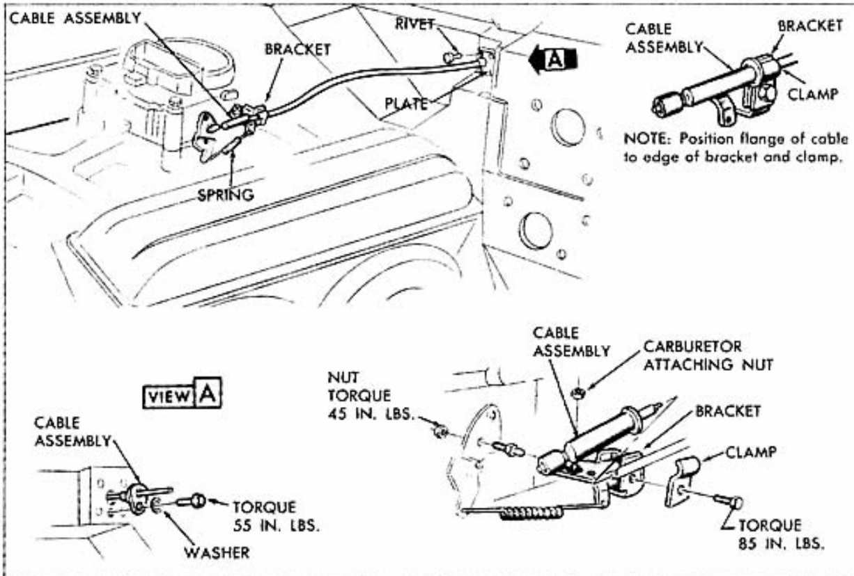
Fig. 5—1970 Corvette Accelerator Controls—8 Cylinder Engines
