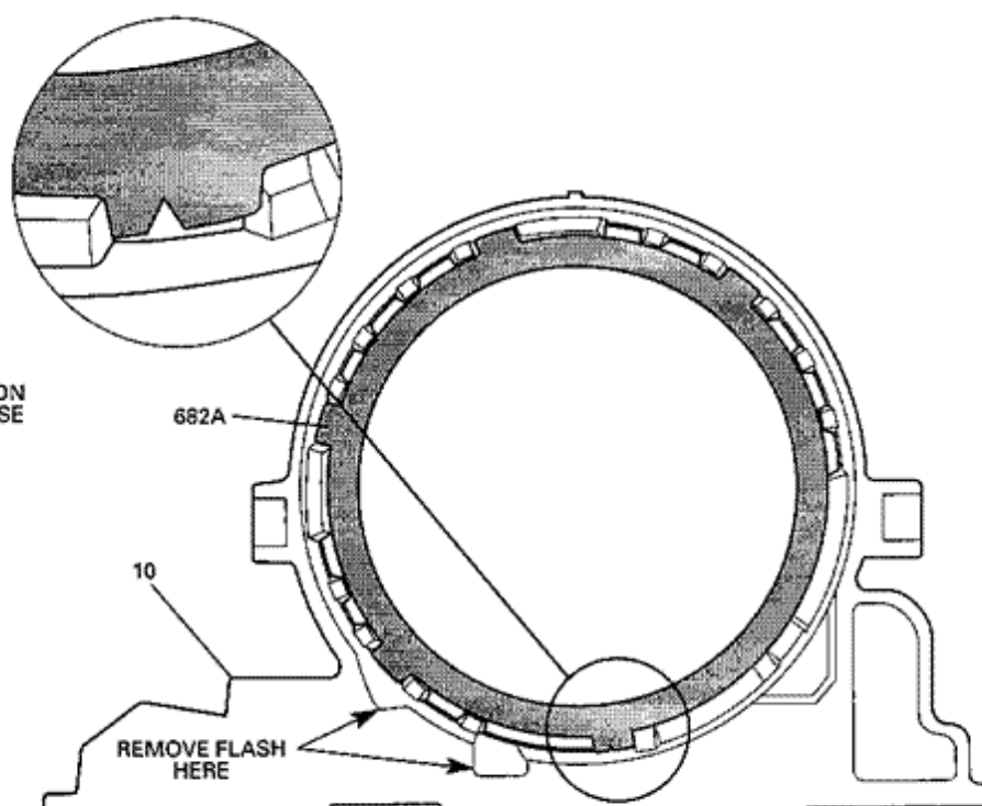
Figure 2 - Lo And Reverse Clutch Waved Plate
