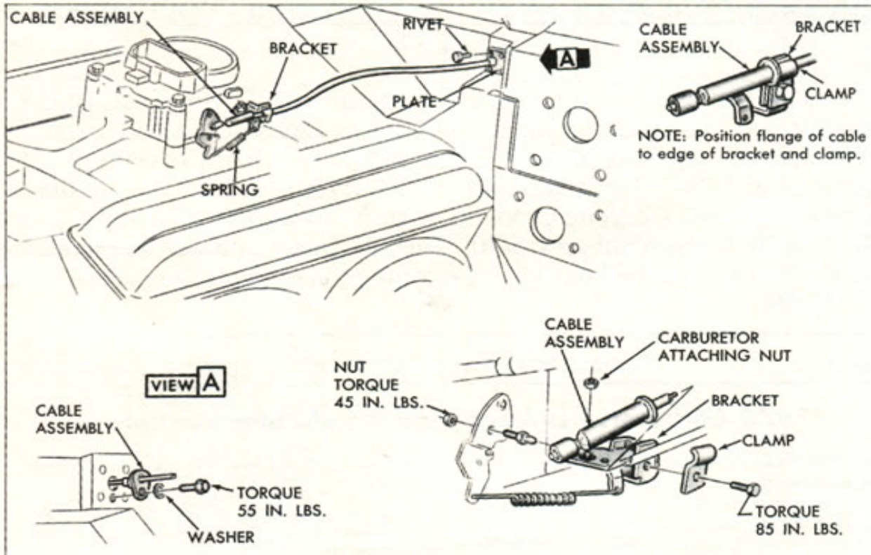
Fig. 5—1970 Corvette Accelerator Controls—8 Cylinder Engines
