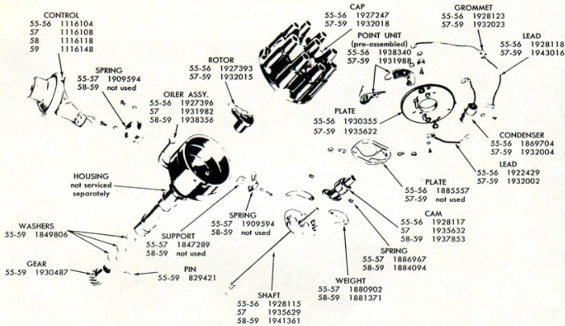
1955-1959 EIGHT CYLINDER IGNITION DISTRIBUTOR (TYPICAL)
