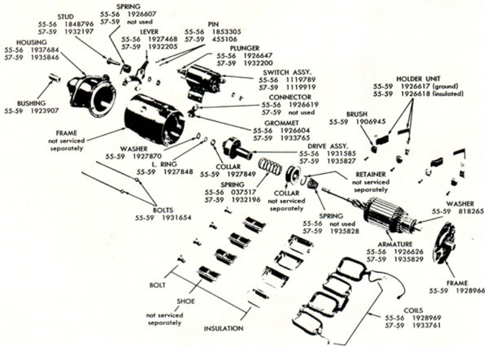
1955-59 STARTING MOTOR-SOLENOID SWITCH (TYPICAL)
