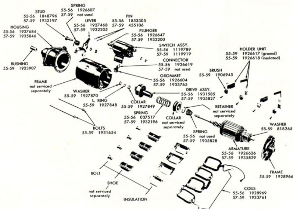
1955-59 STARTING MOTOR-SOLENOID SWITCH (TYPICAL) Standard Eight Cylinder (283)
