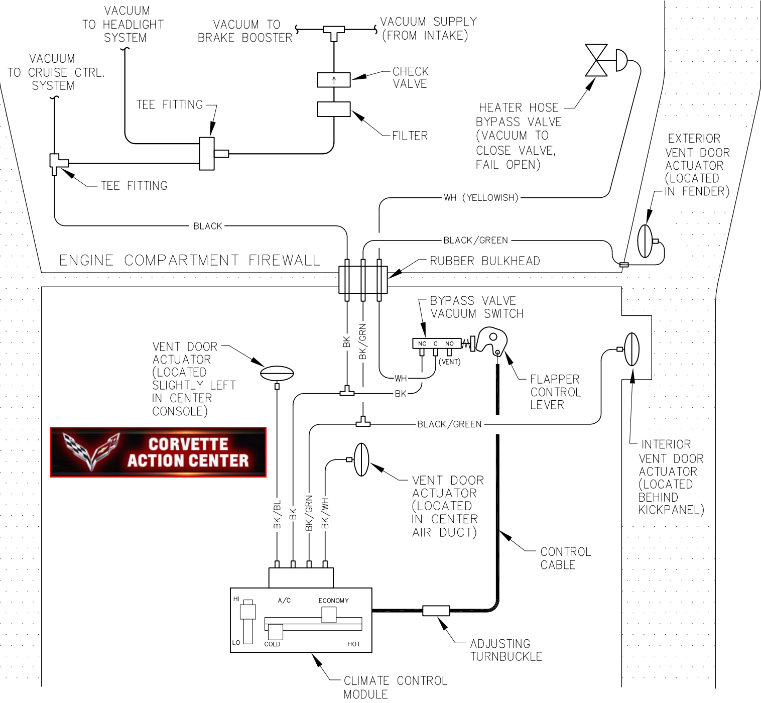
1977 CORVETTE CLIMATE CONTROL VACUUM DIAGRAM (BY VIC RODRIGUE, JR.)
